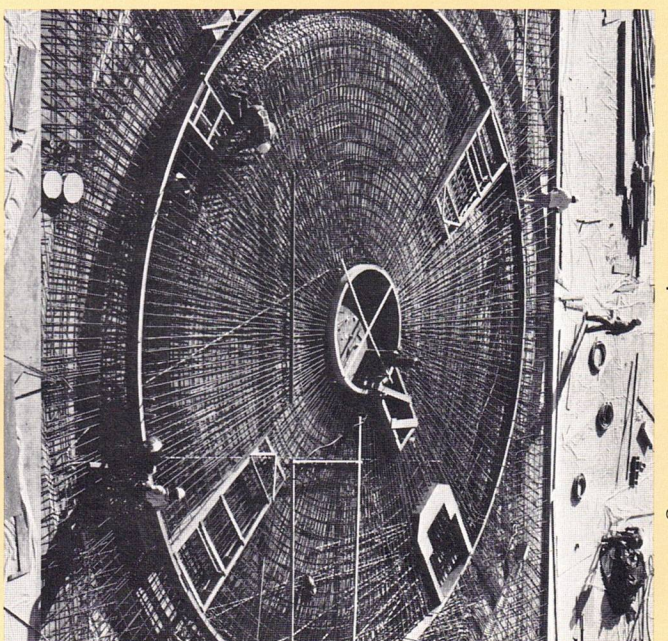
January 1975: Ready for pouring the dome room floor with its radial pattern of reinforcing steel.
